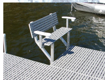
Aluminum Bench with Titan Decking (Bench overhangs water allowing more deck space)
